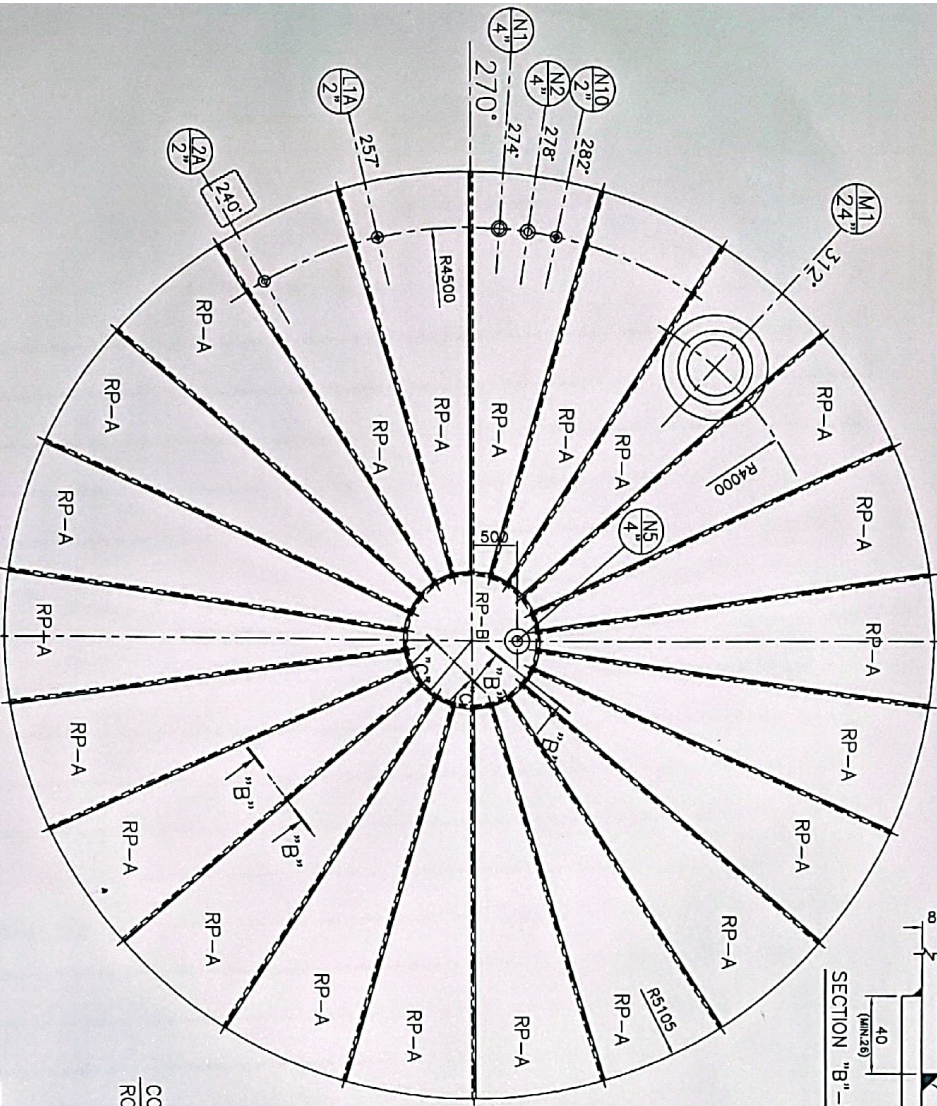
ROOF PLATE DETAIL
