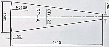
ROOF PLATE DETAIL
