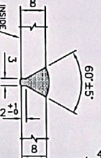
SECTION "C"-C"
